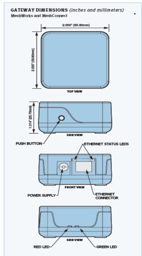
MeshWorks ™ | MeshConnect ™ Ethernet Gateway (ZMx-GW-ETH-1)
